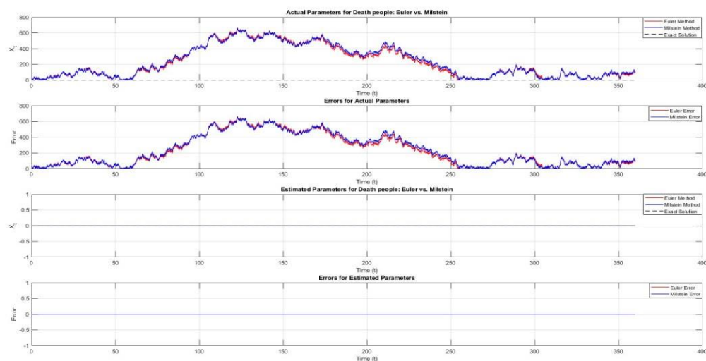
Fig.3. Ornstein-Uhlenbeck processes time series using the Euler and Milstein methods with estimated and actual parameters of death individuals.
