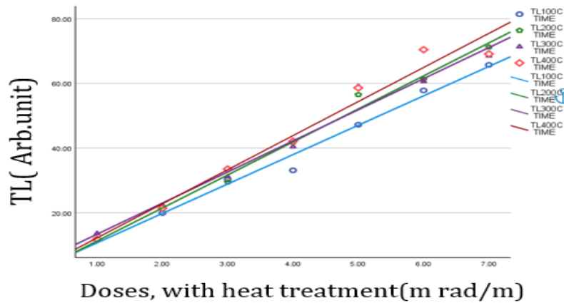
Fig.4. Represents the thermoluminescence resulting from TLD 200 after heat treatment with different doses.
